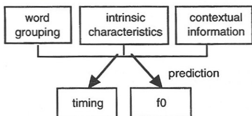
Figure 1. The fundamental structure of prosodic prediction in our system.
